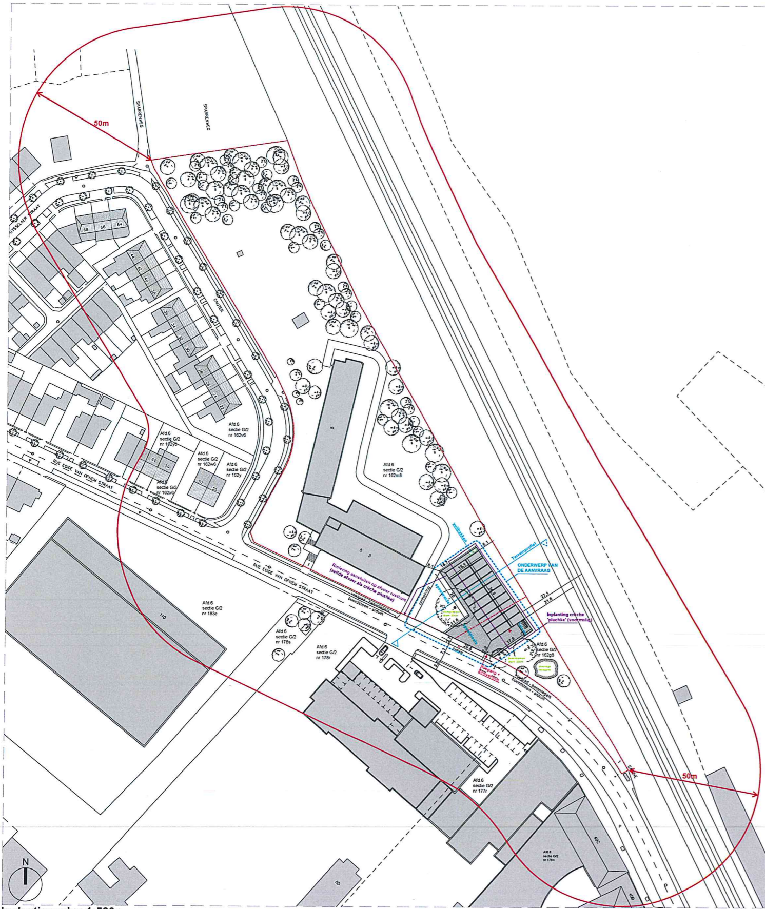
Inplantingsplan 1:500e
